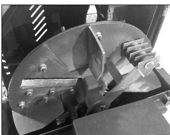
Disc wheel with blades and knife
